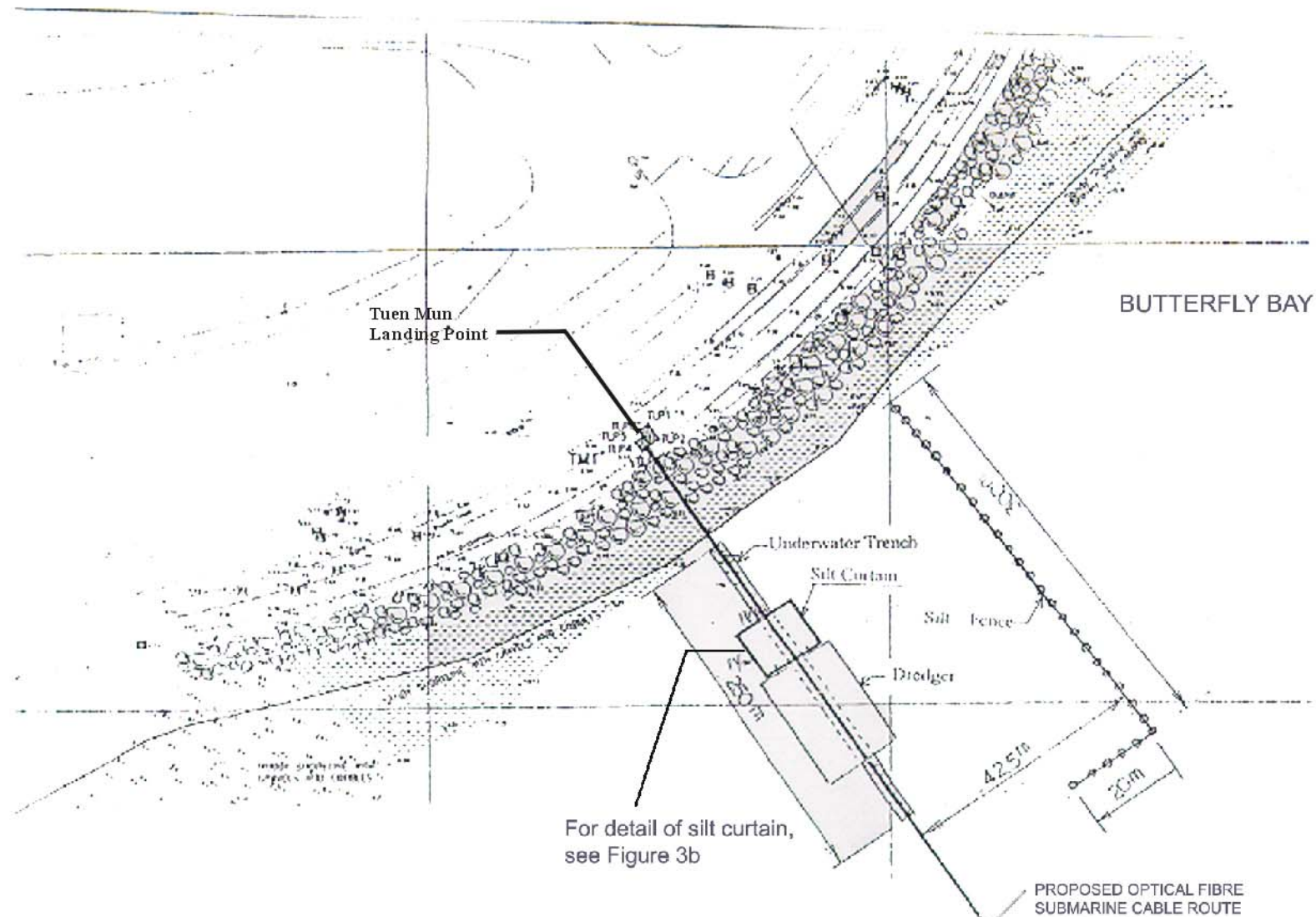
LOCATION OF SILT FENCE DURING THE UNDERWATER TRENCHING AS DESCRIBED IN EP CONDITION 2.3
